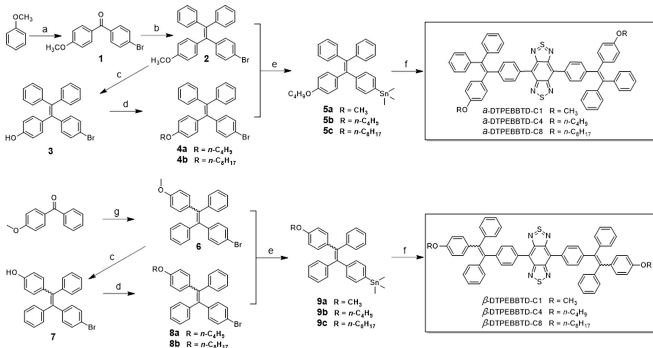
Scheme 1 Chemical structures and synthetic routes to \alpha -DTPEBBTD- C x and \beta -DTPEBBTD- C x . x represents the carbon numbers of the alkoxy chains on the TPE blocks, and x = 1, 4 or 8. Reagents and conditions: (a) \text{AlCl}_3 , 4-bromobenzoyl chloride, \text{CH}_2\text{Cl}_2 , 0–10 °C, overnight; (b) (i) BuLi, diphenylmethane, 0 °C, overnight; (ii) p -toluenesulfonic acid, toluene, 100 °C, 3 h; (c) \text{BBr}_3 , \text{CH}_2\text{Cl}_2 ; (d) \text{Cs}_2\text{CO}_3 , DMF, room temperature, 1-bromobutane for 4a and 8a, 1-bromooctane for 4b and 8b; (e) BuLi, \text{Me}_3\text{SnCl} , THF, –78 °C, overnight; (f) \text{Pd}(\text{PPh}_3)_4 , toluene, 100 °C, 24 h.
