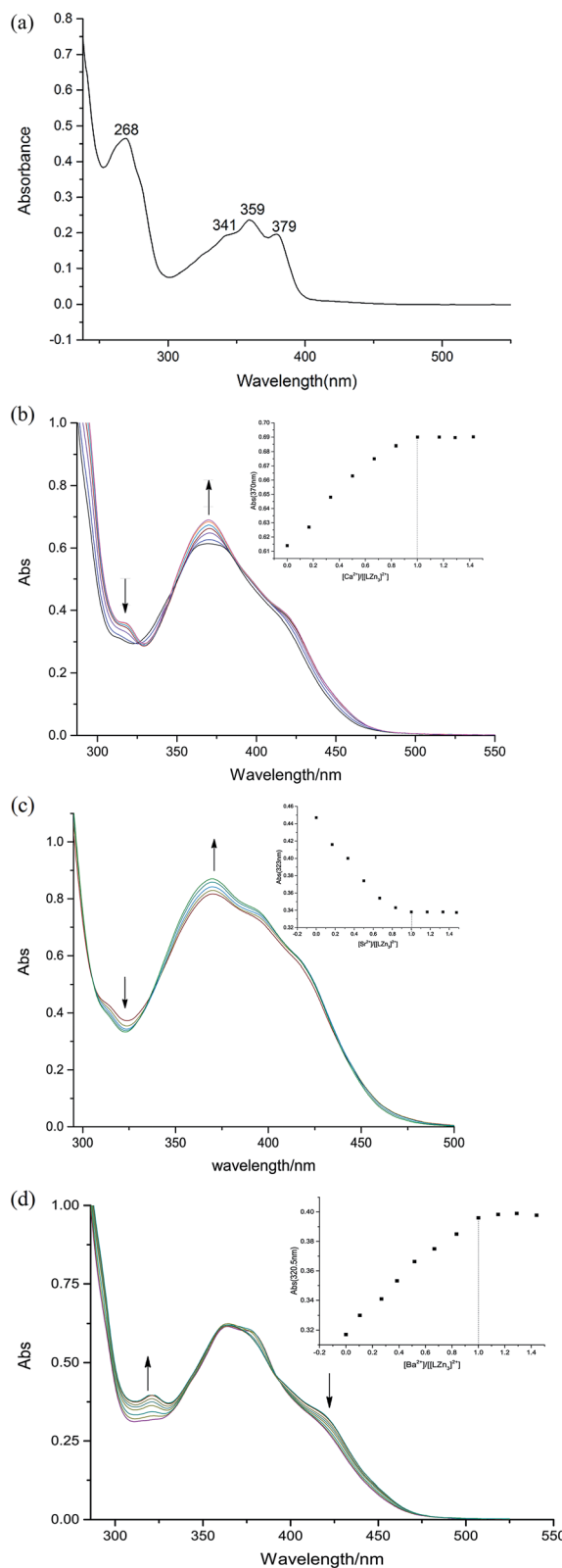
Fig. 2 (a) UV-vis spectrum of the free ligand in \text{CHCl}_3/\text{CH}_3\text{OH} ; (b) the changes in the \text{Zn(II)-L} complex upon addition of \text{Ca(OAc)}_2 \cdot \text{H}_2\text{O} ; (c) the changes in the \text{Zn(II)-L} complex upon addition of \text{Sr(OAc)}_2 \cdot \text{H}_2\text{O} ; (d) the changes in the \text{Zn(II)-L} complex upon addition of \text{Ba(OAc)}_2 .
