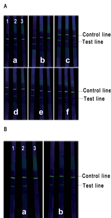
Fig. 6 The stability of strips. 1, 2 and 3 represented the different concentrations of E. coli O157:H7, namely 10^6 CFU mL -1 , 10^5 CFU mL -1 and 10^4 CFU mL -1 , respectively (A) The results of strips for the detection of E. coli O157:H7 after storing for 0 d (a), 7 d (b), 14 d (c), 21 d (d), 28 d (e) and 35 d (f) (B) the diagrams of the used strips after storing for 0 d (a) and 20 d (b).
