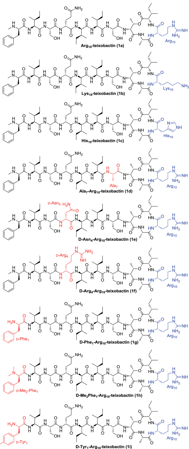
Fig. 2 Structures of teixobactin analogues 1a–i .
