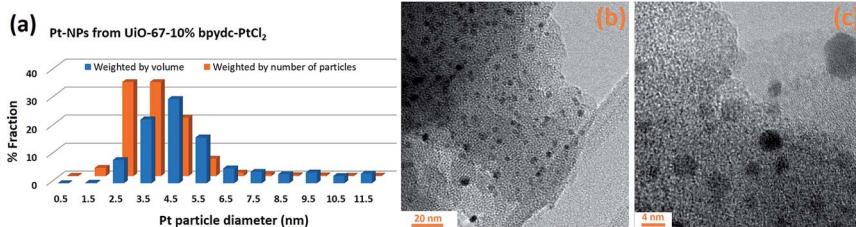
Fig. 7 Part (a): Pt NP distributions (weighted by number of particles (orange) or by volume (blue): w_P(d_i) and w_V(d_i) , respectively, see eqn (3)) obtained from the TEM analysis of the \text{PtCl}_2(\text{H}_2\text{bpydc}) functionalized UiO-67-Pt(II) MOF measured after the \text{H}_2 -TPR XAS experiment reported in Fig. 6. Parts (b) and (c) report two micrographs at different magnifications.
