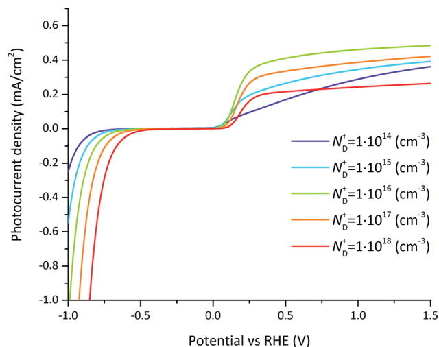
Fig. 10 Photocurrent–voltage curves for varying doping concentration for the reference case (parameters indicated in Tables 1 and 2). For small doping concentrations (below 10^{14} cm -3 ), the photocurrent–potential relation is linear. For intermediate doping concentrations (around 10^{16} cm -3 ), the photocurrent shows an optimum at which the band bending is maximized and recombination is reasonable. At large doping concentrations (above 10^{18} cm -3 ) recombination dominates.
