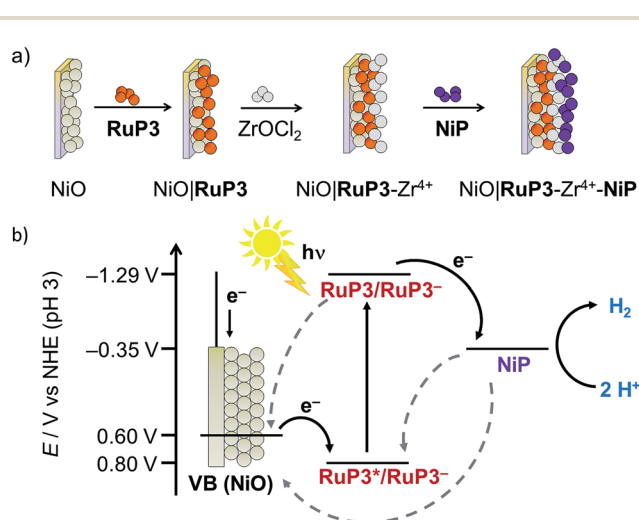
Fig. 2 (a) Supramolecular dye-catalyst assembly on photocathode: layer-by-layer deposition of RuP3 , \text{Zr}^{4+} and NiP on p-type NiO photocathode (see text for details). (b) Energy diagram of the NiO photocathode assembly showing the proposed electron transfer mechanisms (reductive quenching) as black solid arrows and possible recombination pathways as grey dashed arrows between p-NiO, RuP3 and NiP .
