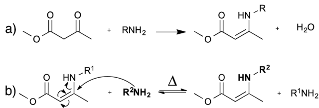
Fig. 5 (a) Synthesis of vinyllogous urethane; this reaction can even be performed in water. (b) Exchange of vinyllogous urethanes and amines occurs at temperatures above 100 °C without catalyst via a Michael addition.
