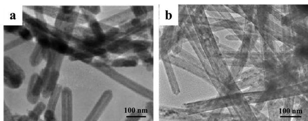
Fig. 2 TEM images of (a) \text{Ce}(\text{OH})_3 nanotubes synthesized at 120 °C, (b) \text{CeO}_2 nanotubes formed during controlled annealing of the \text{Ce}(\text{OH})_3 nanotubes synthesized at 120 °C (modified with permission from ref. 60, copyright 2005 Wiley-VCH).
