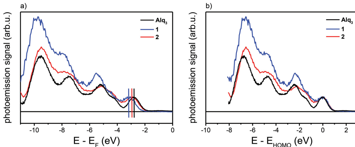
Fig. 7 Left: Comparison between the UPS spectra of \text{Alq}_3 , 1 , and 2 of 4 ML molecules on cobalt. Right: The same spectra, but with the spectral feature from the HOMO of each molecule shifted to the same energy ( E - E_{\text{HOMO}} = 0 eV) for better comparison. The shift (relative to \text{Alq}_3 ) was 0.4 eV for 1 and 0.2 eV for 2 .
