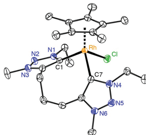
Fig. 2 ORTEP representation of the complex cation complex 7 (50% probability ellipsoids, hydrogens omitted for clarity). Selected bond lengths: Rh–C1 2.026(2) Å, Rh–C7 2.082(2) Å, Rh–Cl 2.410(4) Å, Rh–Cp centroid 1.862(4) Å; selected bond angles: C1–Rh–C7 91.21(9)°; C1–Rh–Cl 96.16(6)°, C7–Rh–Cl 84.74(7)°.
