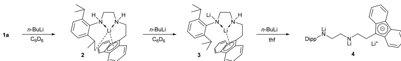
Scheme 2 Lithiation studies of 1a (Dipp = 2,6- i -Pr 2 C 6 H 3 ).
