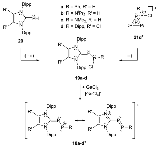
Scheme 7 Two different approaches for the synthesis of NHC stabilized chlorodiphosphanes 19a-d comprising bonding motif B . For 19a,b : (i) +\text{R}'\text{PCl}_2 , +DABCO, -\text{DABCO}\cdot\text{HCl} ; for 19c : (ii) +2\text{PCl}(\text{NMe}_2)_2 , +DABCO, -\text{DABCO}\cdot\text{HCl} , -\text{P}(\text{NMe}_2)_3 ; for 19d : (iii) +3 1,3-bis(2,6-diisopropylphenyl)-4,5-dichloro-imidazole-2-ylidene, 5^+ . Subsequent chloride abstraction yields polarized cationic diphosphenes 18a-d^+ . Only two resonance structures that indicate the polarization of 18a-d^+ are shown.
