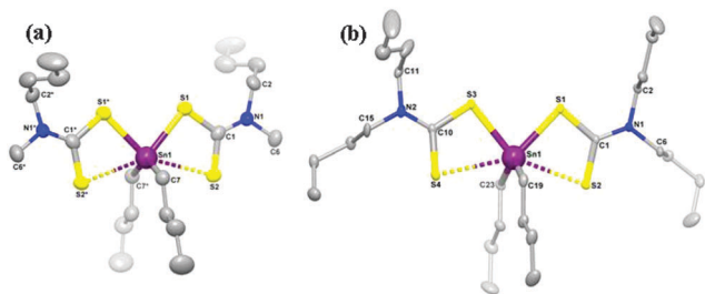
Fig. 10 Molecular structures of (a) [\text{Sn}(\text{C}_4\text{H}_9)_2(\text{S}_2\text{CNMe}'\text{Bu})_2] and (b) [\text{Sn}(\text{C}_4\text{H}_9)_2(\text{S}_2\text{CN}'\text{Bu})_2] with 50% ellipsoidal probability level. All the H atoms on carbon frames are removed for clarity. Reproduced with permission from ref. 97. Copyright 2014 American Chemical Society.
