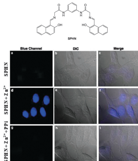
Fig. 43 HeLa cells showed intense blue fluorescence in the presence of both SPHN and Zn 2+ (d) and did not show any fluorescence in the absence of Zn 2+ (a) and in the presence of PPI (g). Corresponding differential interference contrast (DIC) images (e, b and h) and merge images (f, c and i) of the cells are shown. Image reproduced with permission. 194
