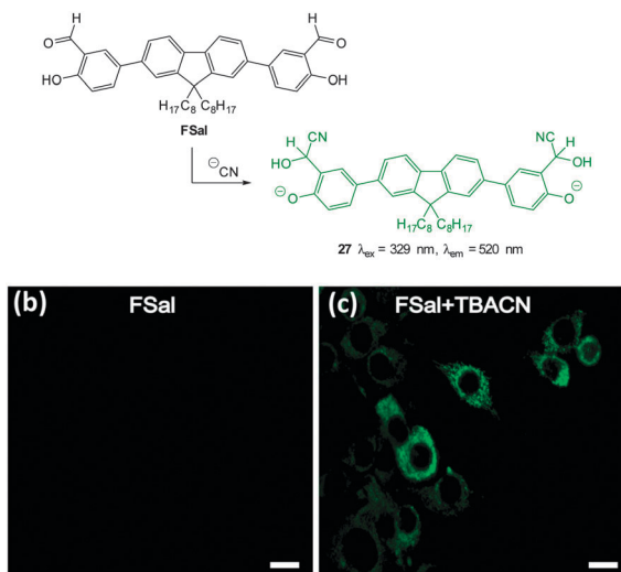
Fig. 27 Top: structure and reaction of fluorene based FSaI with - CN. Bottom: images of SH-SY5Y neuronal cells which were incubated with (left) FSaI alone and (right) FSaI then TBACN. Image reproduced with permission. 173
