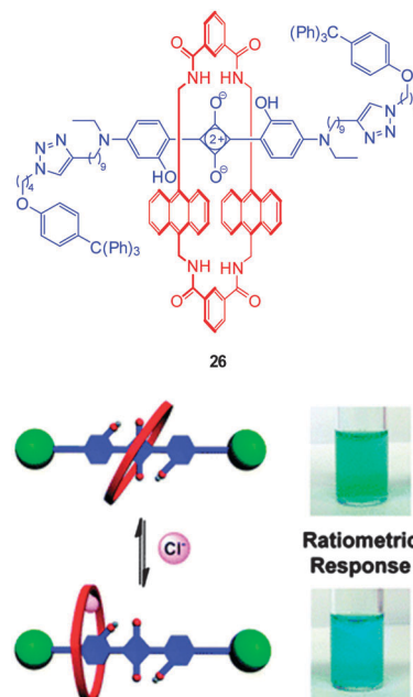
Fig. 23 Fluorescent Cl^- sensor 26 based on a squaraine-rotaxane shuttle. Image reproduced with permission. 166
