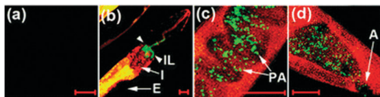
Fig. 34 Top: cyanine based ligand 39. Bottom: imaging of cyanide in C. elegans infected with P. aeruginosa (GFP). Prior to incubation with 39-Cu(II) C. elegans nematodes were fed for 2 d on non-infectious E. coli OP50 (a) or GFP-labelled PA14 (b–d). (b) the anterior end, (c) the medial part, (d) the posterior. (I = intestine; IL = intestinal lumen; I = intestine; E = eggs; PA = PA14-GFP; A = anus). Scale = 20 μm. Image reproduced with permission. 181
