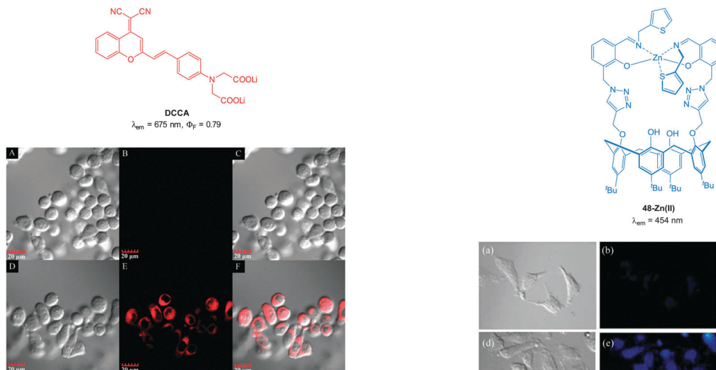
Fig. 41 Top: structure of copper ligand DCCA . Bottom: confocal fluorescence images in KB cells: (A–C) cells incubated with DCCA 2 -Cu(II) alone. (D–F) Cells incubated with DCCA 2 -Cu(II), then K 4 P 2 O 7 . Emission collected at 630–730 nm, excitation at 405 nm. Bright field (A and D), fluorescence (B and E) and overlap field (C and F). Image reproduced with permission. 192
