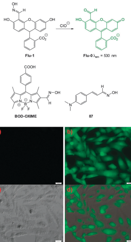
Fig. 89 Top: structure, and reaction of, Flu-1 with \text{ClO}^- . Middle: structures of BOD-OXIME and 87 . Bottom: (a) image of HeLa cells incubated with Flu-1 (20 \mu\text{M} ) for 30 min. (b and c) Fluorescence and bright-field images of cells pre-treated with Flu-1 then incubated with \text{ClO}^- for 30 min. (d) Overlay image of (b) and (c). Image reproduced with permission. 313
