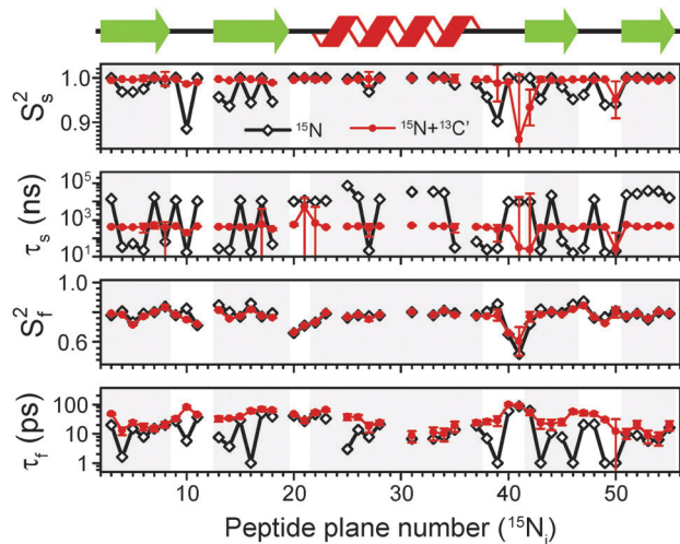
Fig. 5 Comparison of an extended model free (EMF) analysis of backbone dynamics based on ^{15}\text{N} R_1 and R_{1p} relaxation (black line) and combined ^{15}\text{N} R_1 and R_{1p} and ^{13}\text{C}' R_1 and R_{1p} relaxation for the sites in the same peptide planes (red line). S_s^2 , \tau_s , S_f^2 , \tau_f are, respectively: order parameter for the slow motion (reflecting amplitude of motion), correlation time for the slow motion, order parameter for the fast motion and correlation time for the fast motion. Measurements performed both at 600 and 850 MHz spectrometers were used in both cases. The overall amplitude of motion was constrained by measurements of NH dipolar couplings, which are averaged by motions faster than the inverse of its rigid limit value. The data for which NH dipolar couplings were not available or for which severe peak overlap hindered accurate measurement of relaxation rates were excluded.
