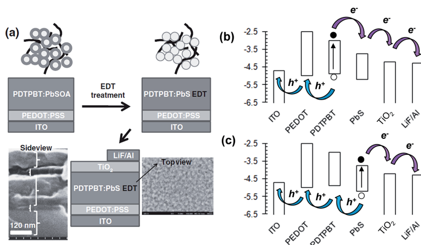
Fig. 11 Hybrid polymer solar cell construction and energy levels. (a) Assembly of EDT-treated PDTPBT:PbS SC. The SEM image shows a side view of the SC photoactive layer. 161 The structure of PDTPBT is shown in Fig. 7. OA and EDT are oleic acid and 1,2-ethanedithiol. (b) Energy level diagram for the SC constructed using values in ref. 161. The arrows used here depict photogeneration of charges from both PDTPBT and PbS. The excitons depicted in (b) were created in the polymer phase; whereas, those depicted in (c) were created in the NC phase. (a) reproduced with permission from ref. 161.
