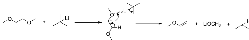
Scheme 25 Reactivity of monoglyme with t -butyllithium.
