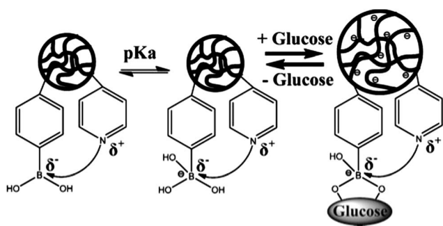
Fig. 3 Illustration for Lewis acid/base interaction in the microgels and glucose-induced swelling. (Reprinted with permission from ref. 38. Copyright © 2011 WILEY-VCH Verlag GmbH & Co. KGaA, Weinheim.)
