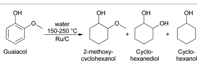
Scheme 1 The reaction pathway for the catalytic hydrotreatment of quaiacol with Ru/C. 29
