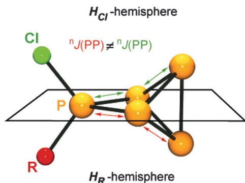
Fig. 9 Definition of the H_{Cl} - and H_R -hemisphere in cations 32a–h + . The tetra-coordinated P atoms span a plane. The tri-coordinated P atom above the plane is within the H_{Cl} -hemisphere, and the P atom below the plane is in the H_R -hemisphere.
