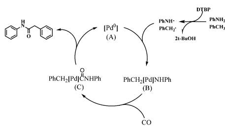
Scheme 3 The proposed reaction mechanism.
