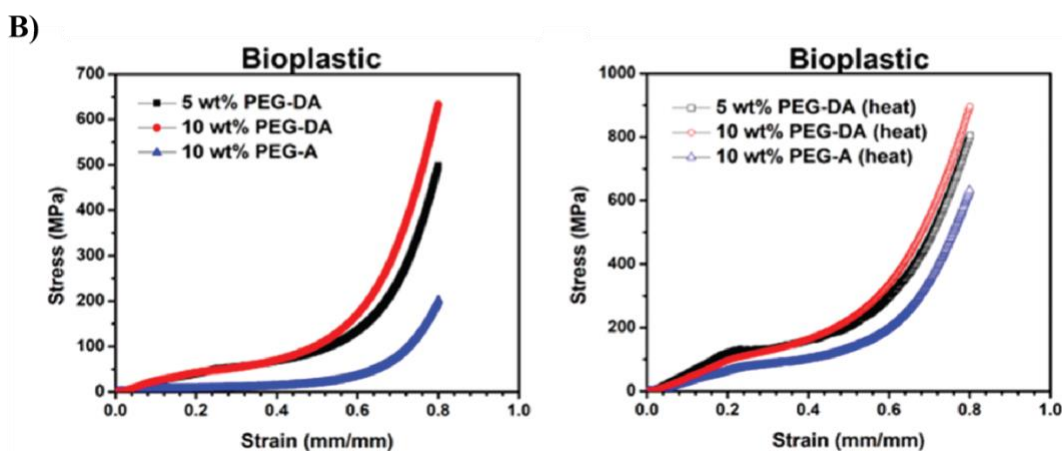
Figure 18: A) (a) Schematic of the 3D printing process and post processing steps. (b) Resin composition (BSA: bovine serum albumin) (c) Schematic depicting network structure after photopolymerization. (d) Network structure after heating to denature the protein. 71 B) Compressive stress vs strain curves for BSA mixed with either PEG di-acrylate (PEG-DA) or PEG acrylate (PEG-A) for the material as a hydrogel (left graph) and the material after heat treatment denaturing the protein (right graph). 71 Reprinted with permission from {P. T. Smith, B. Narupai, J. H. Tsui, S. C. Millik, R. T. Shafrank, D.-H. Kim and A. Nelson, Additive Manufacturing of Bovine Serum Albumin-Based Hydrogels and Bioplastics, Biomacromolecules , 2020, 21 , 484–492} Copyright {2020} American Chemical Society.
