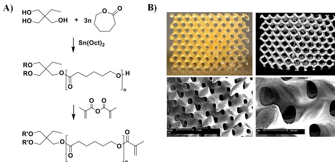
Figure 9: A) Synthesis of three-armed PCL macromers (Reproduced from Elomaa et.al.). 31 B) Photograph, microcomputed tomography visualization, and SEM images of SLA printed PCL scaffolds. 31 Reprinted from Acta Biomater. , Vol 7, L. Elomaa, S. Teixeira, R. Hakala, H. Korhonen, D. W. Grijpma, J. V. Seppälä, Preparation of poly( \epsilon -caprolactone)-based tissue engineering scaffolds by stereolithography, 3850–3856, Copyright (2011), with permission from Elsevier.
