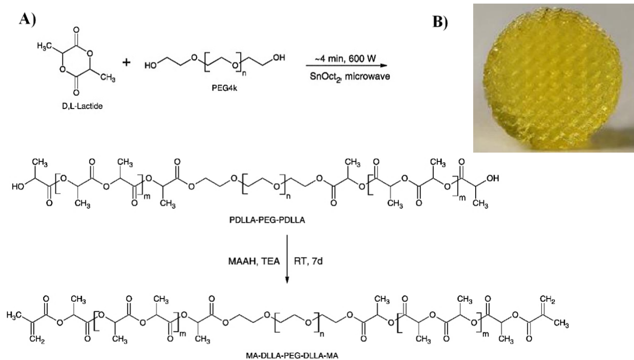
Figure 26: A) Synthesis of PDLLA-PEG-PDLLA triblock copolymers, followed by end functionalization with methacrylic anhydride (MAAH) to install methacrylate groups. 84 B) Photograph of hydrogel scaffold with gyroid pore network. The diameter of hydrogel disk is 8 mm. 84 Reprinted from J. Control. Release , 148, T. M. Seck, F. P. W. Melchels, J. Feijen, D. W. Grijpma, Designed biodegradable hydrogel structures prepared by stereolithography using poly(ethylene glycol)/poly(d,l-lactide)-based resins, 34–41, Copyright (2010), with permission from Elsevier.
