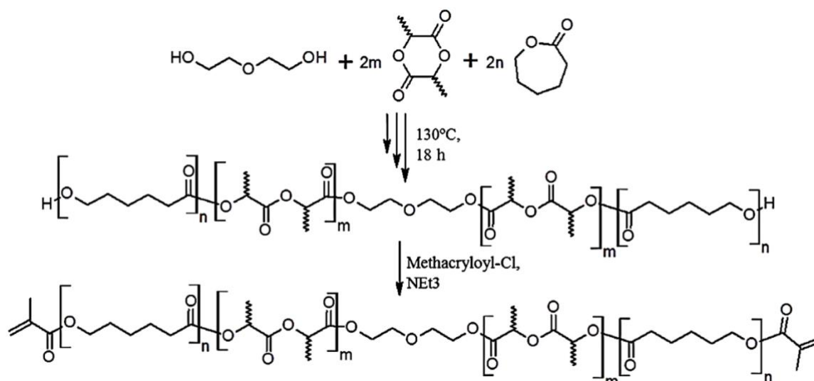
Figure 29: Synthesis of PLA-PCL random copolymers followed by methacrylation. 39 Reproduced from R. M. Felfel, L. Pooza, M. Gimeno-Fabra, T. Milde, G. Hildebrand, I. Ahmed, C. Scotchford, V. Sottile, D. M. Grant and K. Liefelth, In vitro degradation and mechanical properties of PLA-PCL copolymer unit cell scaffolds generated by two-photon polymerization, Biomed. Mater. , 11, 015011, 1 st December 2015, DOI: 10.1088/1748-6041/11/1/015011. Copyright © IOP Publishing. Reproduced with permission. All rights reserved.
