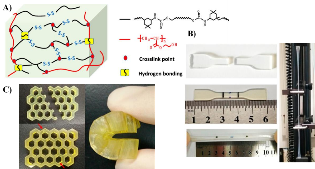
Figure 34: A) Schematic depicting the synthetic strategy of disulfide bonds based self-healing materials. 93 B) Images depicting self-healing of tensile test specimens. The specimens are cut into two parts, healed at 80 °C for 12 hrs, and then stretched to a large deformation. 93 C) Self-healing of the DLP printed honeycomb structure. The honeycomb structure was cut into two parts, healed at 80 °C for 12 hrs, and then could be freely bent. 93 Reprinted with permission from {X. Li, R. Yu,
