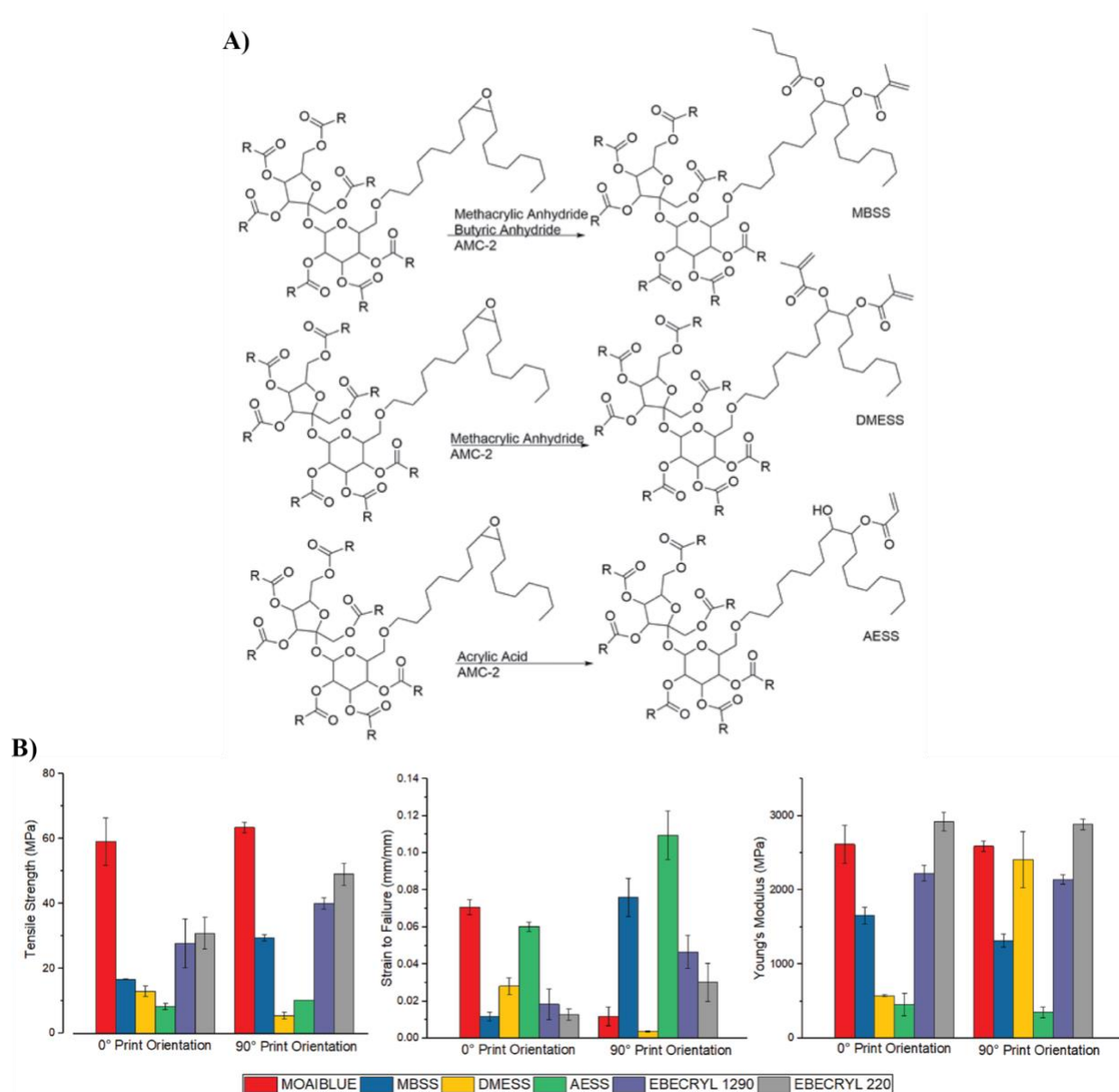
Figure 7: A) Synthesis of sucrose-based resins MBSS, DMESS, and AESS for SLA printing. 30
