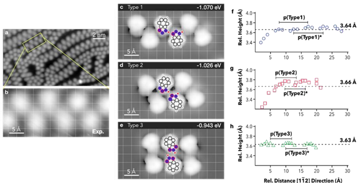
Fig. 4. a) STM image after annealing to 308 K, 18.7 \times 10.2 \text{ nm}^2 , 1.033 V, 0.077 nA; b) magnification of the yellow rectangle in a). c-e) Simulated STM images for the hexameric chains, 1 V, constant current. A grid to guide the eye and a model representation are superposed to each simulated image. Top-right, adsorption energy per molecule; f-h) Extrapolated N atoms positions projected along the [11\bar{2}] direction.
