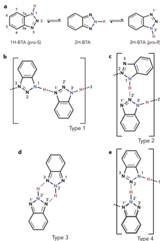
Scheme 1 Benzotriazole ( C_6H_5N_3 , BTAH) chemical structure and tautomeric equilibrium (a). Some of the possible basic dimeric structures based on hydrogen bonds: b) the N_1-H \cdots N_1' linkage, c) the N_1-H \cdots N_2' linkage, d) the N_3-H \cdots N_2' + N_2-H \cdots N_3' double linkage, e) the N_2'-H \cdots N_2 linkage. Atoms are labelled for ease of description and discussion.
