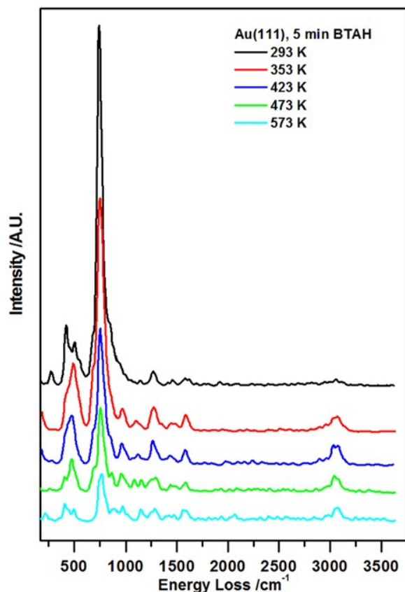
Fig. 1. Enhanced HREEL spectra of as prepared BTAH on clean Au(111) and spectra evolution with annealing.
