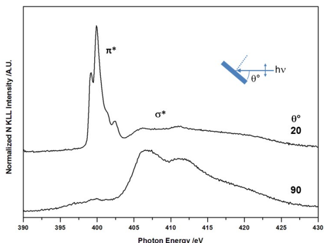
Fig. 2. As prepared angular dependent NEXAFS N K-edge spectra at saturation coverage, collected at 298 K.
