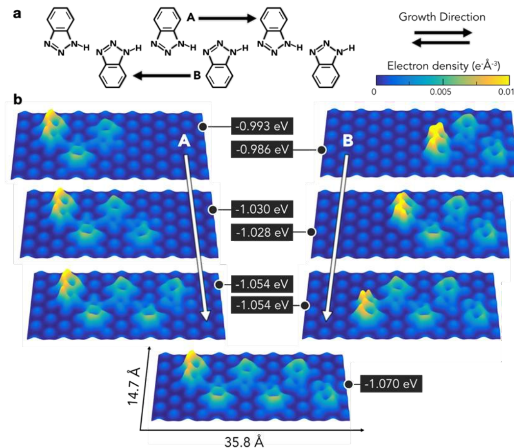
Fig. 5. a) Chemical representation of the type 1 chains modelled. A and B arrows indicate the growth direction. b) Electron density of the different chains projected on a plane parallel to the surface at a distance of 2.0 Å. Adsorption energies are normalised by the number of BTAH molecules adsorbed.
