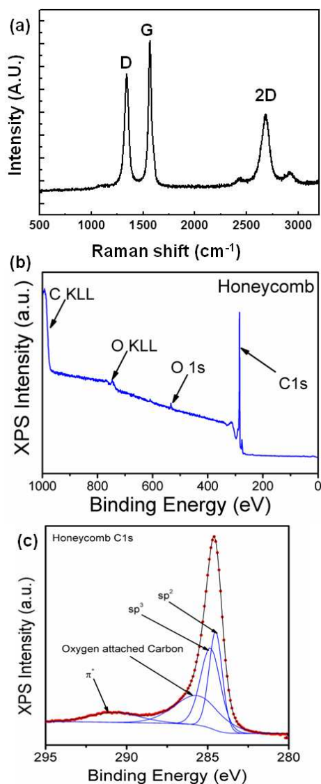
Figure 2: (a) Raman spectrum of HC-VGS. (b) XPS survey scan and (c) C 1s narrow scan of HC-VGS. Spectrum was fitted with the sp^2 , sp^3 , oxygen-attached carbon, and \pi - \pi^* shake-up features.
