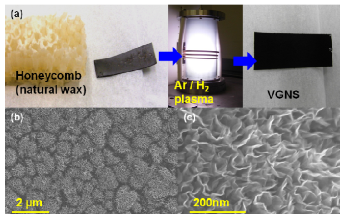
Figure 1: Transformation of honeycomb (natural wax) into vertical graphenes in a reactive Ar + \text{H}_2 plasma-based process. (a) Honeycomb was liquefied on the graphite paper substrate which was placed in an ICP-CVD system, whereupon a short plasma exposure was utilized to reform the honeycomb precursor and grow the HC-VGS. As-grown HC-VGS on flexible graphite substrate with supporting (b) SEM; and (c) high-resolution SEM images featuring its morphology.
