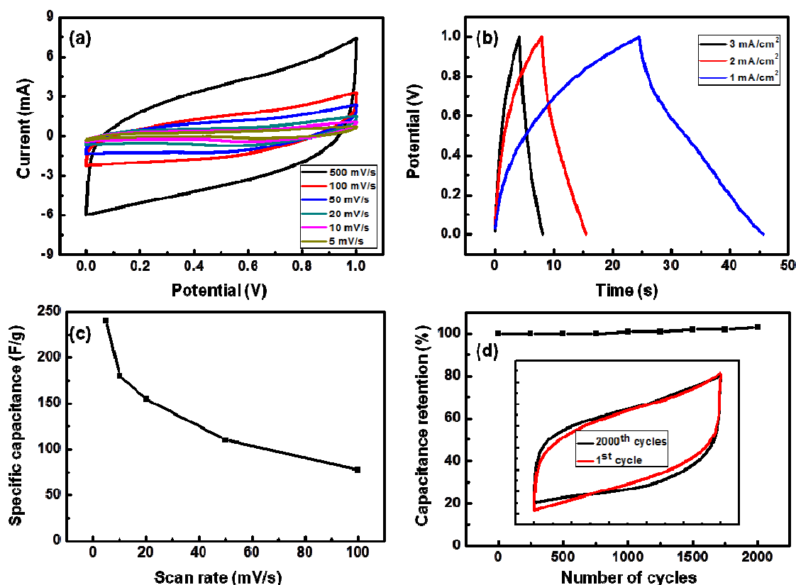
Figure 3: Supercapacitor performance of HC-VGS. CV curves of (a) HC-VGS at different scan rates of 5, 10, 20, 50, 100 mV/s and 500 mV/s. (b) Galvanostatic charge/discharge plots of HC-VGS at current densities of 3, 2 and 1 mA/cm 2 . (c) Rate capabilities of HC-VGS, and (d) cycle stability of HC-VGS at a scan rate of 400 mV/s for 2000 cycles.
