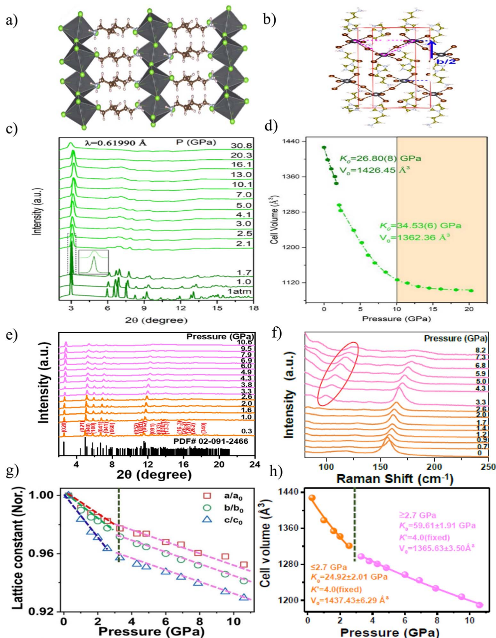
Fig. 6 Pressure-induced structural changes in DJ-type 2D HOIPs with rigid spacers. (a) Crystal structure at ambient pressure of (2meptH 2 )PbCl 4 . Reproduced from ref. 34 with permission from the Royal Society of Chemistry, copyright 2023. (b) Crystal structure at ambient pressure of (API)PbBr 4 . Reproduced from ref. 46 with permission from Wiley-VCH GmbH, copyright 2024. (c) and (d) In situ ADXRD spectra upon compression to 30.8 GPa and unit cell volume as a function of pressure of (2meptH 2 )PbCl 4 . Reproduced from ref. 34 with permission from the Royal Society of Chemistry, copyright 2023. (e)–(h) In situ XRD spectra upon compression to 10.6 GPa, Raman spectra upon compression to 8.2 GPa, normalized unit cell parameters as functions of pressure, and unit cell volume as a function of pressure of (API)PbBr 4 . Reproduced from ref. 46 with permission from Wiley-VCH GmbH, copyright 2024.
