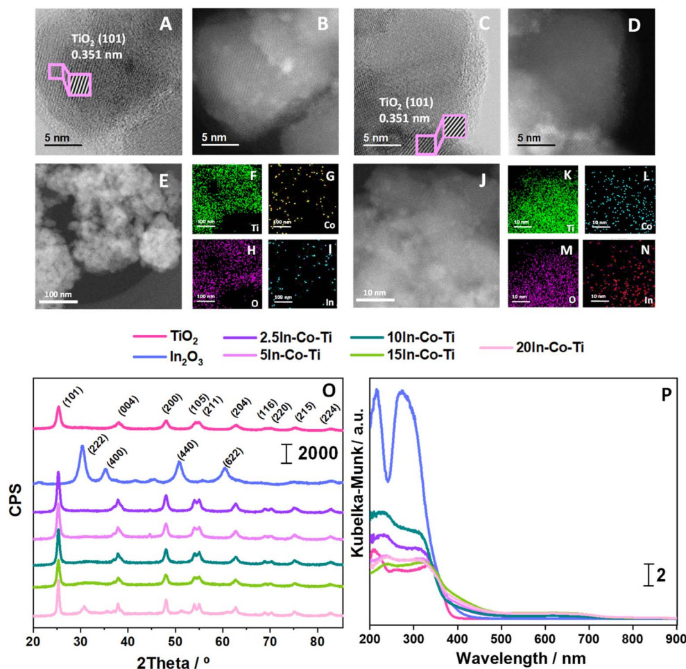
Fig. 2 (A and B) TEM micrographs for the 2.5In-Co-Ti sample. (C and D) TEM micrographs for the 10In-Co-Ti sample. (E–I) Dark-field STEM (E) and EDS mapping for the 2.5In-Co-Ti sample. (J–N) Dark-field STEM (J) and EDS mapping for the 10In-Co-Ti sample. (O) XRD patterns for the xIn-Co-Ti and reference samples. (P) UV-visible plot spectra for the xIn-Co-Ti samples.
