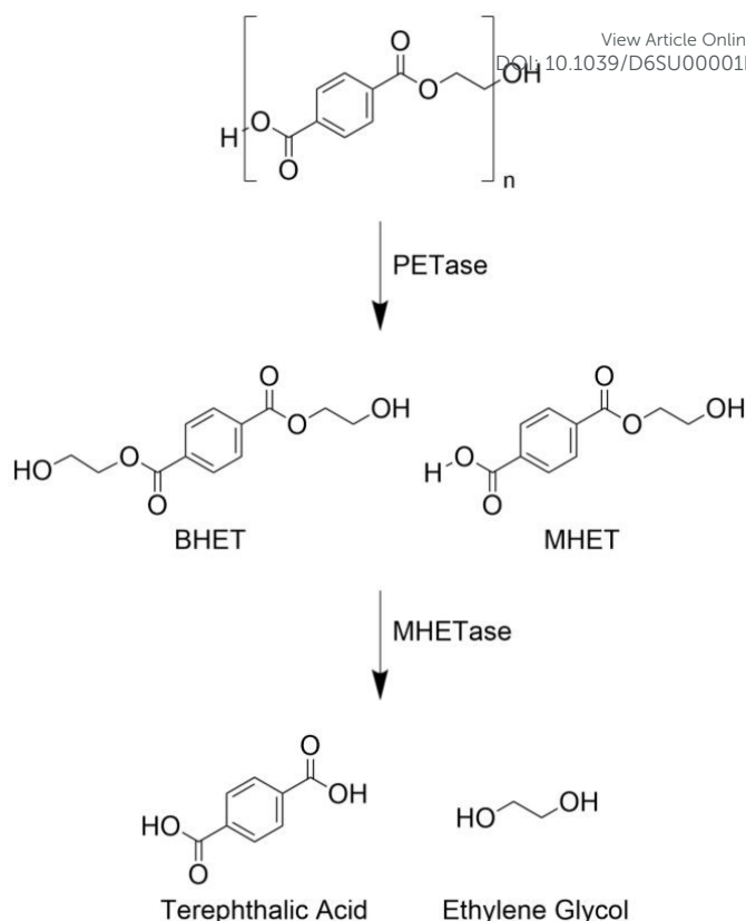
Figure 4. The enzyme-aided depolymerization of poly(ethylene terephthalate) (PET). PETase chops up PET into smaller units including bis(2-hydroxyethyl) terephthalate (BHET) and mono(2-hydroxyethyl) terephthalate (MHET). Allowing MHETase to finish the depolymerization producing terephthalic acid and ethylene glycol.
