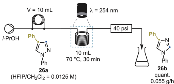
Scheme 7 Reaction scale-up using photo-flow equipment. a Reaction conducted at 0.025 M instead of 0.0125 M. nd: not determined.
