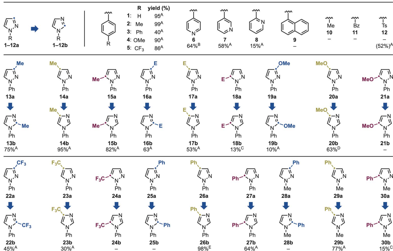
Scheme 3 Substrate scope for the pyrazole-to-imidazole conversion using mono-substituted derivatives. E = CO 2 Me. The yield for substrate 12 corresponds to the desilylated product.
