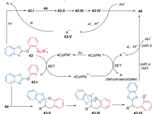
Scheme 16 Intermolecular radical difunctionalization by docking-migration of arylbenzothiazolyether reagents.
