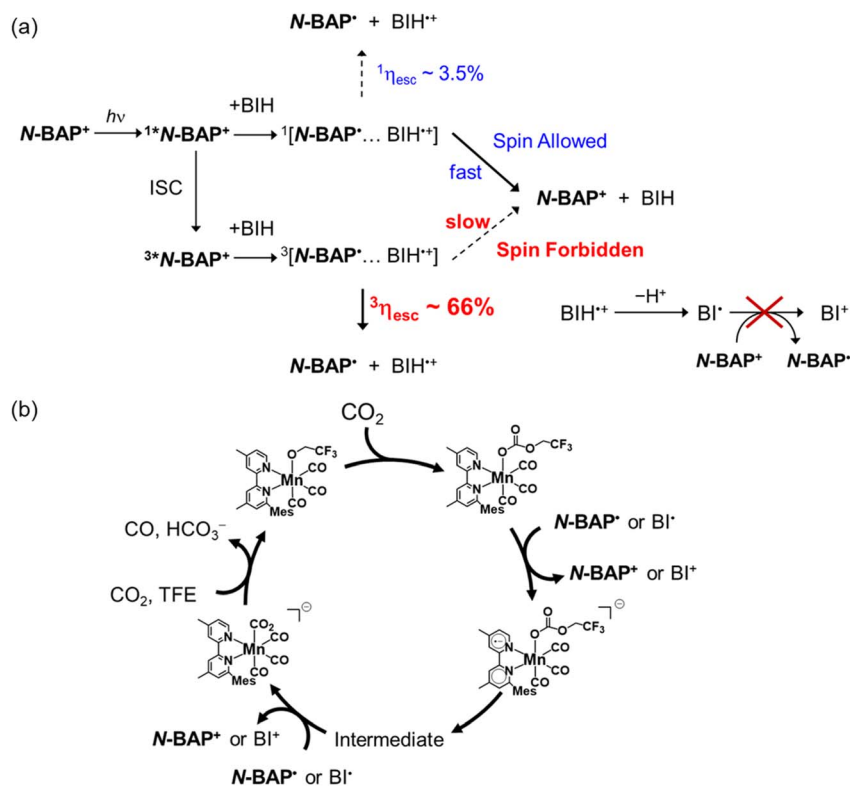
Scheme 4 Mechanism of the photocatalytic \text{CO}_2 reduction reaction: (a) reductive quenching processes of 1^*N\text{-BAP}^+ and 3^*N\text{-BAP}^+ by \text{BIH} , and (b) \text{CO}_2 reduction on the Mn-complex catalyst through electron injection processes from the reductive quenching processes.
