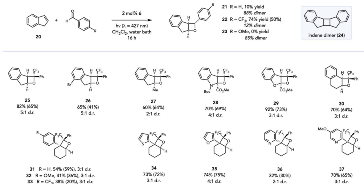
Fig. 4 Scope studies for transposed Paternò–Büchi reactions of indenes and arylcyclohexenes. Assay yields and d.r. determined by crude ^1\text{H} NMR analysis using \text{CH}_2\text{Br}_2 as an internal standard. Isolated yields of the combined diastereomers reported in parentheses.
