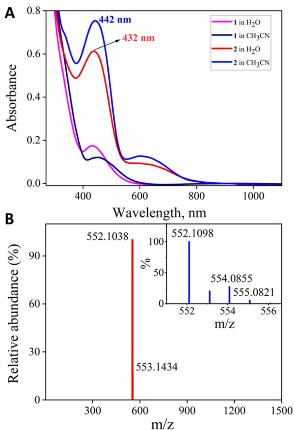
Fig. 2 (A) UV-vis spectra of 2 , both in 100% \text{CH}_3\text{CN} and water from 1 at RT. (B) Negative mode HRMS spectrum of 2 (0.05 mM) in water and mass spectrum of 2 in \text{H}_2\text{O}^{18} (inset).
