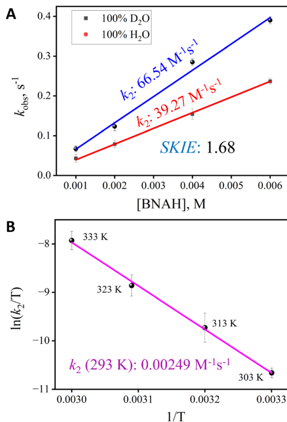
Fig. 3 (A) Plot of the k_2 value for the reaction of 2 (0.05 mM) with varying [\text{BNAH}] at 293 K, in \text{H}_2\text{O} and \text{D}_2\text{O} , to determine the solvent kinetic isotope effect. (B) Determination of k_2 at 293 K for reaction of 2 (0.05 mM) with BNAH in pure acetonitrile solvent from the Eyring plot.
