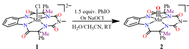
Scheme 1 Schematic diagram for the synthesis of complex (\text{Et}_4\text{N}) [\text{Mn}^{\text{V}}(\text{O})(\text{Ph},\text{Me}-\text{bTAML})] , 2 from 1 .
