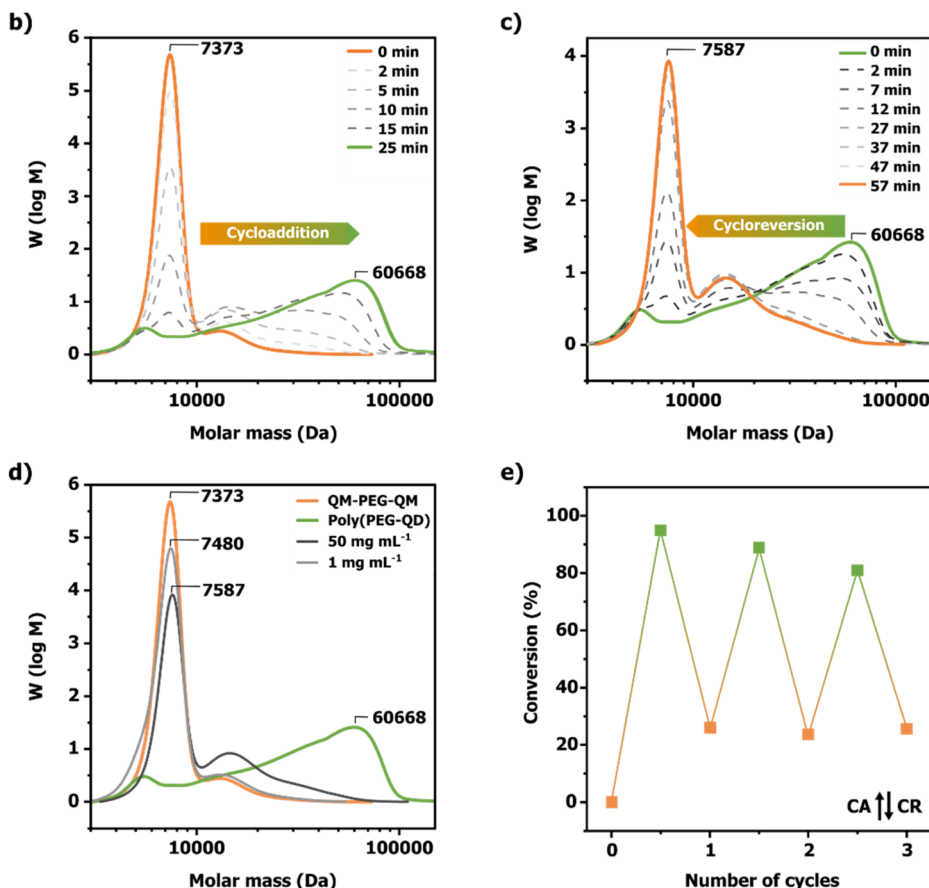
Fig. 4 (a) Schematic representation of the reversible formation of poly(PEG-QD) through an orthogonally triggered [2π + 2π] photocycloaddition (340 nm) and photocycloreversion (265 nm) under oxygen-free conditions. (b) GPC chromatograms from the [2π + 2π] photocycloaddition of QM-PEG-QM ( c = 50 mg mL -1 ), conducted at 340 nm under oxygen-free conditions, at different irradiation times. (c) GPC chromatograms from the [2π + 2π] photocycloreversion of poly(PEG-QD) ( c = 50 mg mL -1 ), conducted at 265 nm under oxygen-free conditions, at different irradiation times. (d) GPC chromatograms from the [2π + 2π] photocycloreversion of poly(PEG-QD), conducted at 265 nm under oxygen-free conditions, at c = 50 mg mL -1 (grey) and at c = 1 mg mL -1 (black). (e) Subsequent irradiation cycles of QM-PEG-QM ( c = 50 mg mL -1 ) conducted at 340 nm (25 min) for cycloaddition (CA, from orange to green) and at 265 nm (45 min) for cycloreversion (CR, from green to orange), under oxygen-free conditions. The photoreactions were carried out in ACN solutions using an LED photoreactor at power levels ranging from 22 to 33 mW.
