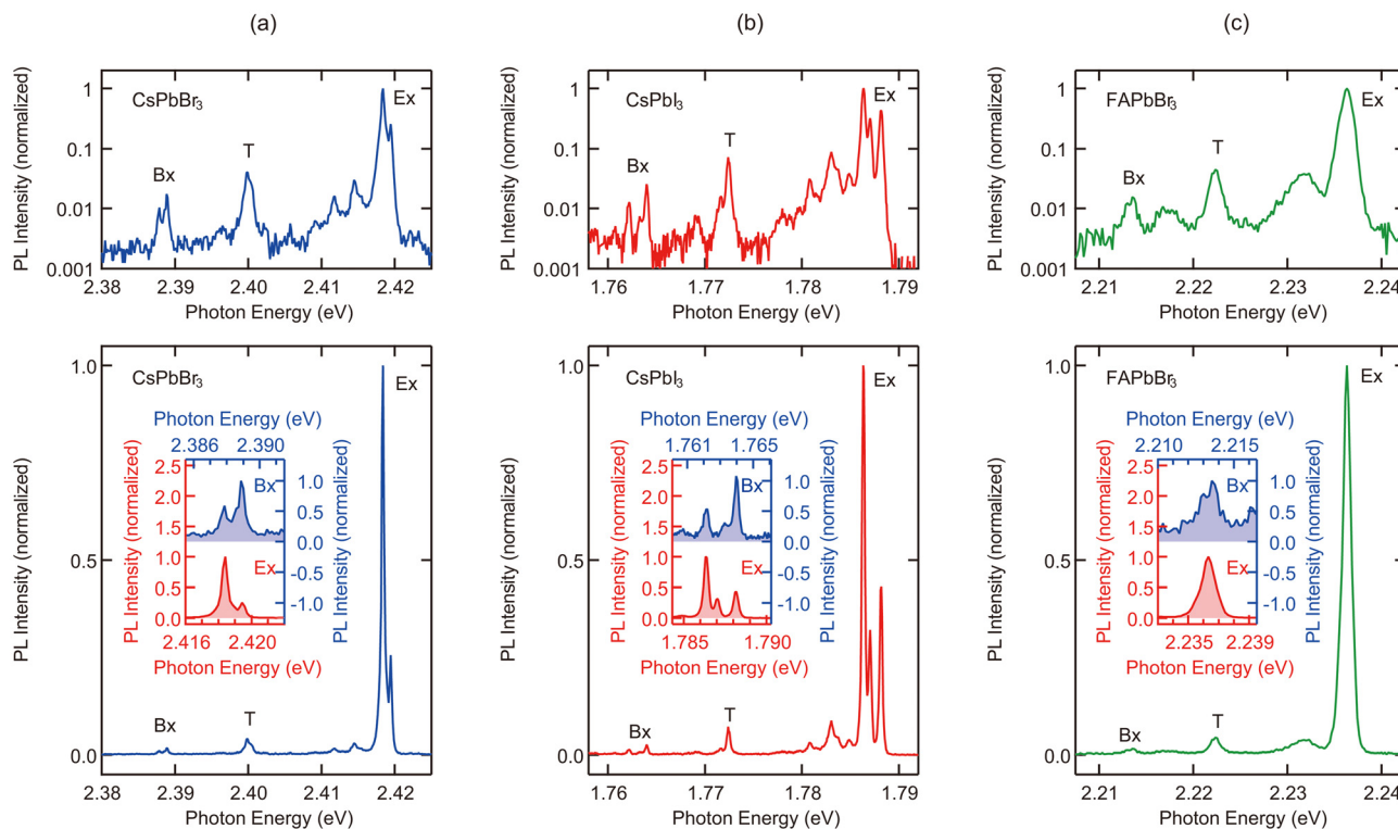
Fig. 2 Representative PL spectra of single (a) CsPbBr 3 , (b) CsPbI 3 , and (c) FAPbBr 3 NCs at 5.5 K. Upper and lower panels are shown in logarithmic and linear scales, respectively. Inset shows comparison of the fine structure splitting of the exciton (red) and biexciton (blue) peaks. Reproduced with permission from ref. 87, © American Chemical Society 2024.
