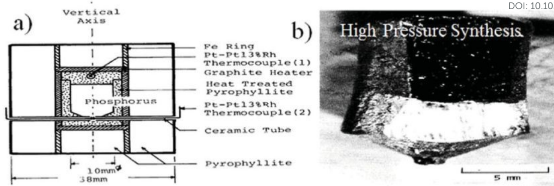
Fig. 5: (a) Growth of black phosphorus (BP) crystals under high pressure and high temperature conditions. (b) Optical image of a BP crystal showing distinct and well-defined crystal faces. Adapted from ref. XX, Nat. Nanotechnol. , 2014, 9, 372–377. This figure is reused in an Open Access publication with appropriate acknowledgment [60].
