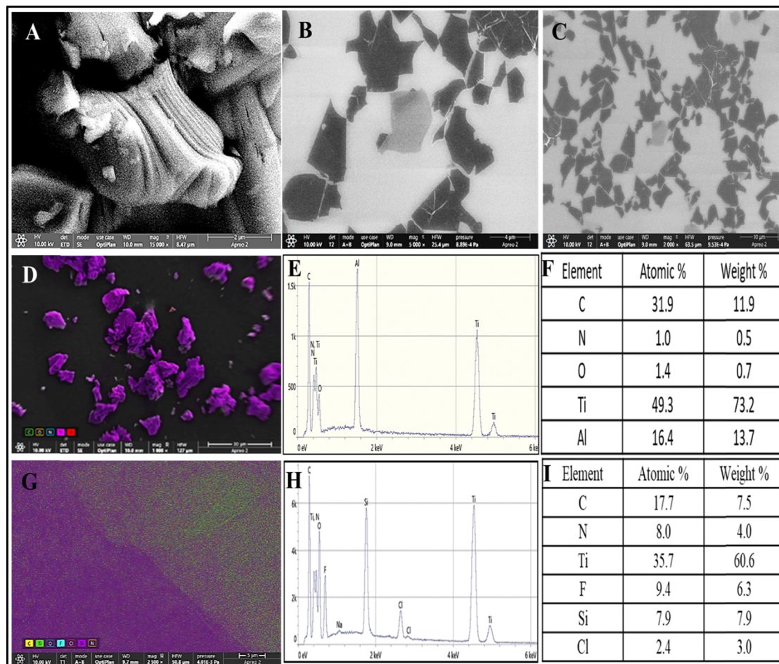
Fig. 2 Microscopic characterization of MXene: HR-SEM for (A) the Max phase ( \text{Ti}_3\text{AlC}_2\text{X} ) and (B) and (C) delaminated MXene sheets ( \text{Ti}_3\text{C}_2\text{X} ); EDS analysis: (D) EDS image, (E) EDS mapping, and (F) elemental composition of the Max phase ( \text{Ti}_3\text{AlC}_2\text{X} ); (G) EDS image, (H) EDS mapping, and (I) elemental composition of delaminated MXene sheets ( \text{Ti}_3\text{C}_2\text{X} ).
