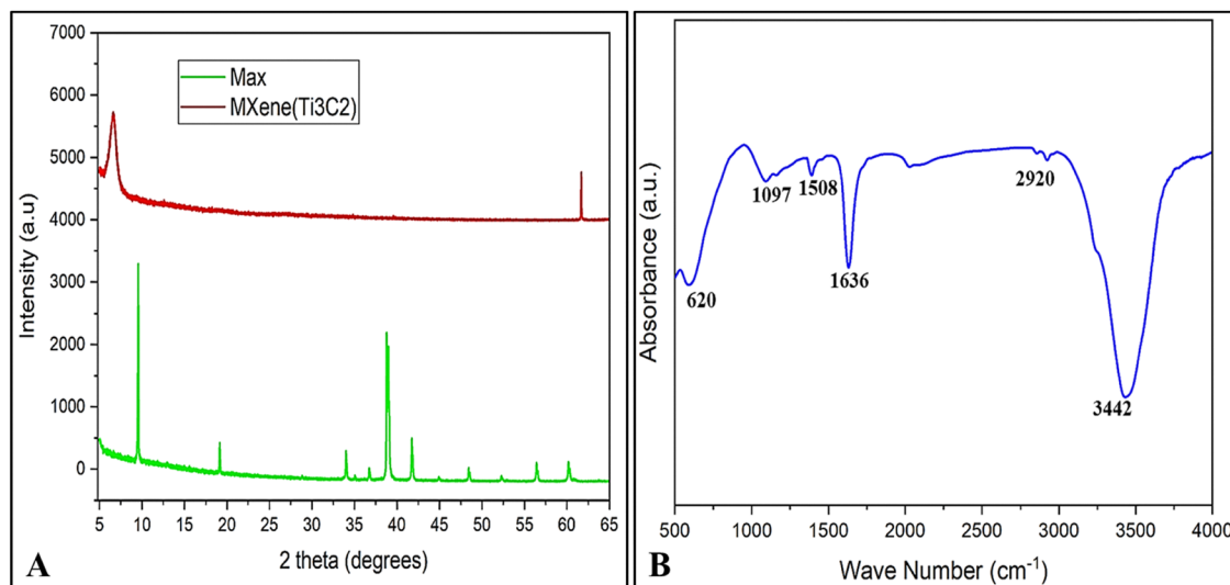
Fig. 3 Characteristics study: (A) XRD of the Max phase ( \text{Ti}_3\text{AlC}_2\text{X} ) and delaminated MXene sheets ( \text{Ti}_3\text{C}_2\text{X} ) and (B) FTIR of delaminated MXene sheets ( \text{Ti}_3\text{C}_2\text{X} ).
