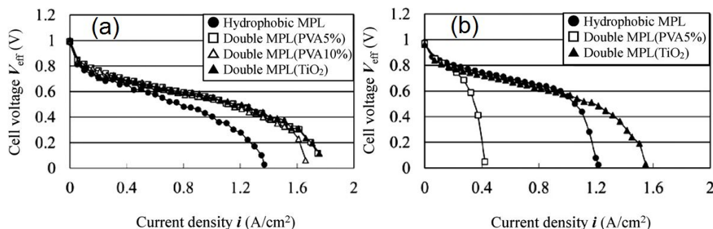
Fig. 16 (a) Influence of hydrophilic layer in double MPL coated GDL (hydrophobic intermediate MPL: 20 mass% PTFE, d_m = 3 \mu\text{m} , h_{\text{PTFE}} = 90 \mu\text{m} ) on PEFC performance under (a) low humidity (anode: 60% RH, cathode: 0% RH) and (b) high humidity (anode: 100% RH, cathode: 100% RH). Reproduced from Ref. 121, copyright 2013, with permission from Elsevier.
