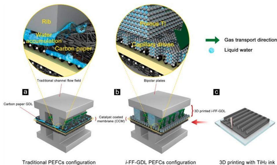
Fig. 14 Schematic diagram of traditional PEMFC configuration (a), i-FF-GDL PEMFC configuration (b) and the 3D printing process (c). Reproduced from Ref. 115, copyright 2021, with permission from Elsevier.
