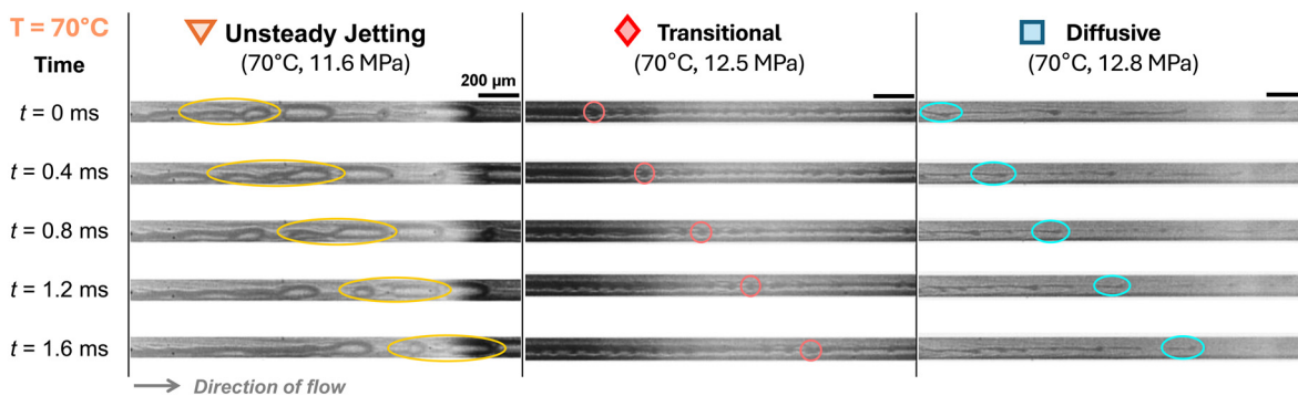
Fig. 6 Time-lapse snapshots at T = 70 °C showing the evolution of the \text{CO}_2 jet tip at 11.6 MPa (unsteady jetting), 12.5 MPa (transitional), and 12.8 MPa (diffusive). Scale bars: 200 \mu\text{m} .
