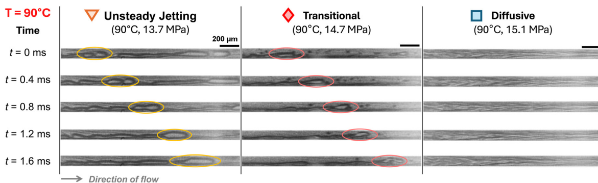
Fig. 7 Time-lapse snapshots at T = 90 °C showing the evolution of the \text{CO}_2 jet tip at 13.7 MPa (unsteady jetting), 14.7 MPa (transitional), and 15.1 MPa (diffusive). Scale bars: 200 \mu\text{m} .
