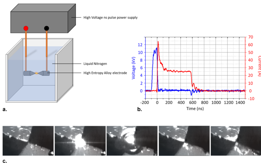
Fig. 1 Experimental setup and discharge dynamics for HEA nanoparticle synthesis via electric discharge in liquid nitrogen. (a) Schematic of the pin-to-pin electrode configuration with high-voltage pulse power supply and liquid nitrogen medium. (b) Voltage (blue) and current (red) profiles during a discharge event, showing a rapid rise time of 30 ns. (c) High-speed camera sequence (30 000 fps) capturing plasma ignition between the electrodes, followed by vapor-bubble formation, expansion, and collapse within tens of microseconds.
