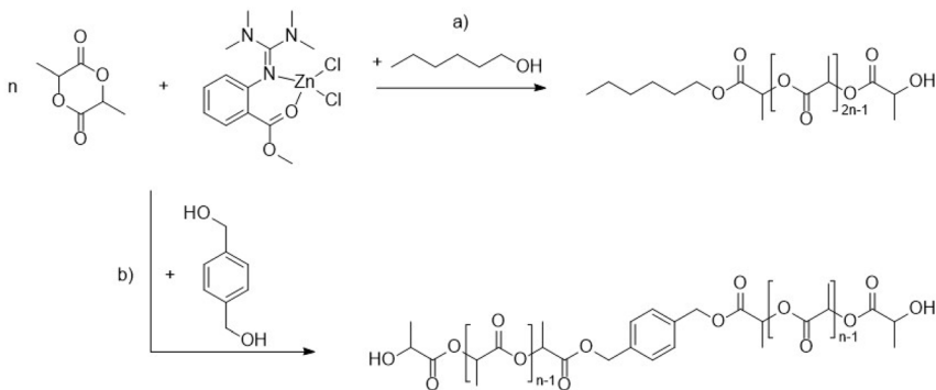
Scheme 1 Lactide ROP catalysed by [ZnCl 2 (TMGasme)] (C1) with two different co-initiators: (a) 1-hexanol (CoI1); (b) 1,4-benzenedimethanol (CoI2).
