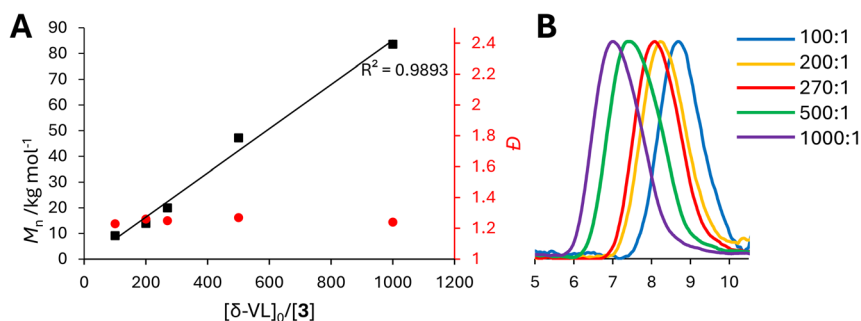
Fig. 2 (A) Plot showing the relationship between M_n of PVL (black squares) and D (red circles) with varying [\delta\text{-VL}]_0/[3] ; (B) GPC traces of PVL at various [\delta\text{-VL}]_0 : [3] ratios.
