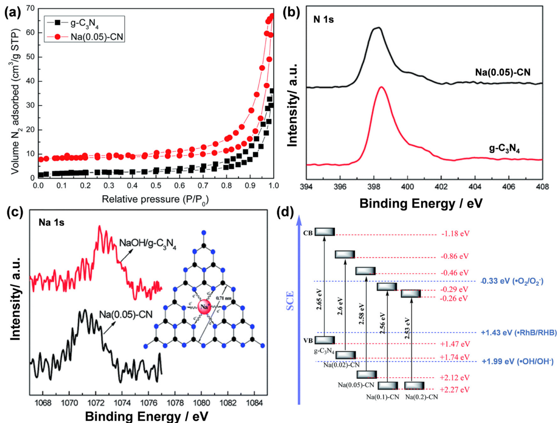
Fig. 11 (a) BET adsorption isotherm of g\text{-C}_3\text{N}_4 and \text{Na}(0.05)\text{-CN} , (b) N 1s, (c) Na 1s XPS spectra (possible doping site of \text{Na}^+ (inset)) of \text{Na}(0.05)\text{-CN} , and (d) band gap structures of the prepared materials. Reproduced with permission from ref. 84. Copyright 2014, Royal Society of Chemistry.
