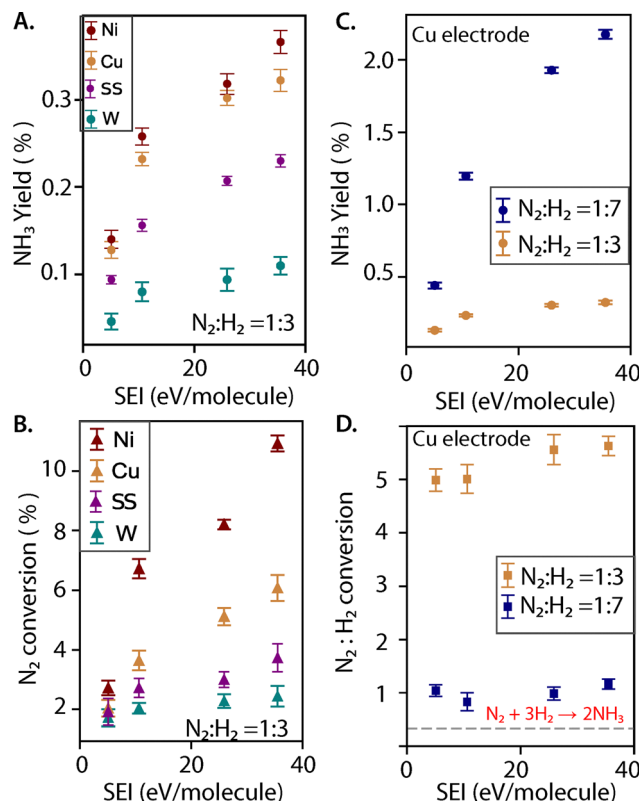
Fig. 5 Effect of electrode material and feed composition on plasma NH 3 synthesis. (A) NH 3 yield SEI for Ni, Cu, and W electrodes at a fixed N 2 :H 2 ratio of 1:3. Ni delivers the highest yield, Cu is intermediate, and W the lowest, despite identical discharge conditions. (B) Corresponding N 2 conversion follows the same order. (C) On Cu, changing feed composition from N 2 :H 2 = 1:3 to 1:7 produces a strong enhancement in NH 3 yield. (D) N 2 :H 2 conversion ratios exceeded the stoichiometric 1:3 requirement (gray dash line), especially in N 2 rich feeds, consistent with electrode nitridation and direct nitrogen incorporation into the metal surface.
