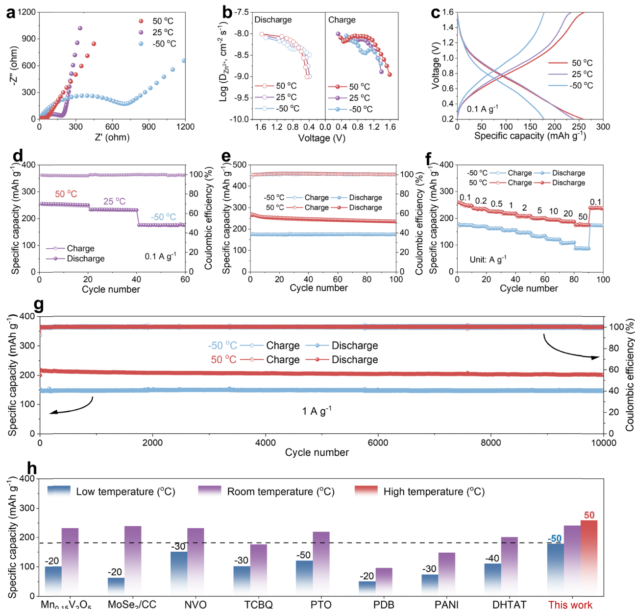
Fig. 5 Electrochemical performance of the PMPZ cathode for AZIBs at high and low temperatures. (a) EIS plots of PMPZ at 50 °C, 25 °C, and -50 °C. (b) Zn 2+ diffusion coefficients of the PMPZ cathode at 50 °C, 25 °C, and -50 °C. (c) Typical charge/discharge curves of PMPZ at 0.1 A g -1 at 50 °C, 25 °C, and -50 °C. (d) Electrochemical performance of PMPZ across a wide temperature range from -50 °C to 50 °C. (e) Cycling performance of PMPZ at 0.1 A g -1 at 50 °C and -50 °C. (f) Rate performance of PMPZ at different current densities and at 50 °C and -50 °C. (g) Long-term cycling performance of PMPZ at 1 A g -1 at 50 °C and -50 °C. (h) Comparison of the specific capacity among PMPZ and previously reported cathode materials at different temperatures.
