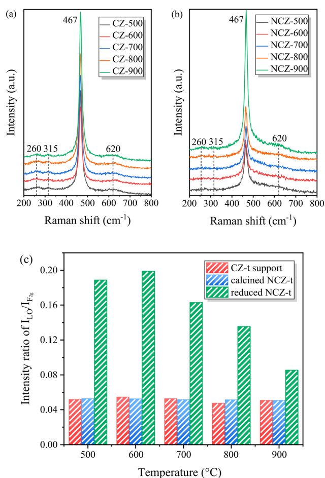
Fig. 5 Raman spectra for (a) the CZ-T supports and (b) the reduced NCZ-T catalysts and (c) the corresponding I_{\text{LO}}/I_{F_{2g}} values.
