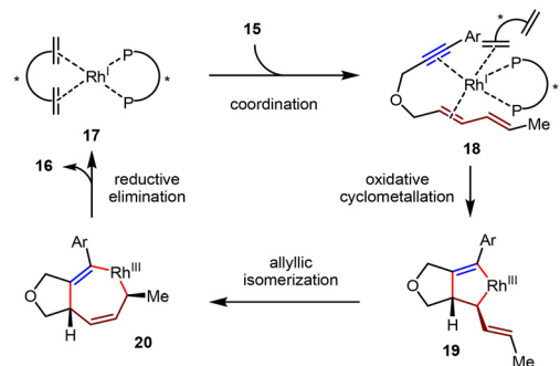
Scheme 9 Asymmetric intramolecular [4+2] cycloadditions catalyzed by a rhodium(I)/DUPHOS/diene complex.
