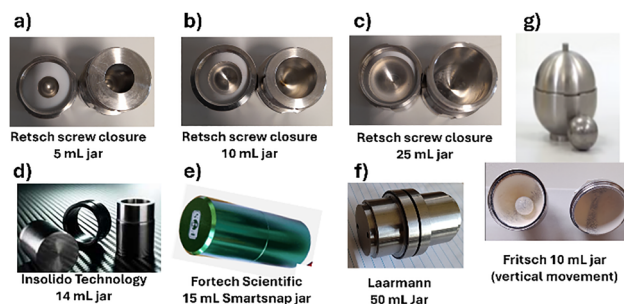
Fig. 3 Commercially available jars used for vibrational ball milling. The internal shape of the top and bottom caps are hemispheres, connected through a cylindric section. (a)–(f) Used under horizontal vibratory motion using ball mills depicted in Fig. 2(b). The milling jar in (g) is used for vertical motion using ball mills depicted in Fig. 2(c).
