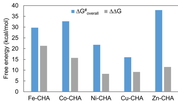
Fig. 4 Overall Gibbs free energy barrier ( \Delta G_{\text{overall}}^{\ddagger} ) and selectivity parameter ( \Delta\Delta G ) for the acetylene hydrogenation to ethylene on M-CHA calculated at 453.15 K.
