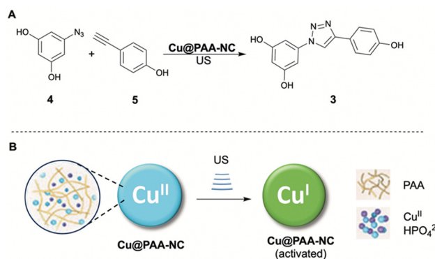
Fig. 13 (A) Formation of resveratrol analogue 3 via Cu@PAA-NC catalyzed CuAAC after catalyst activation with ultrasound (US). (B) Schematic representation of Cu@PAA-NC and its activation mechanism using US. 98 Partly reproduced from ref. 98 with permission from Wiley.
